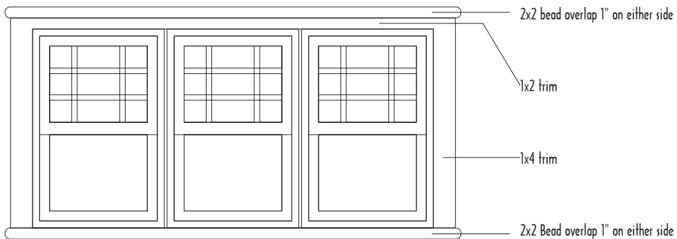
Typical 2nd Floor Exterior Window Trim
