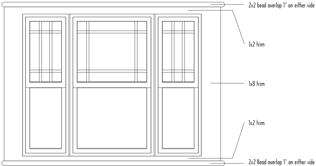
Typical 1st Floor Exterior Window Trim
