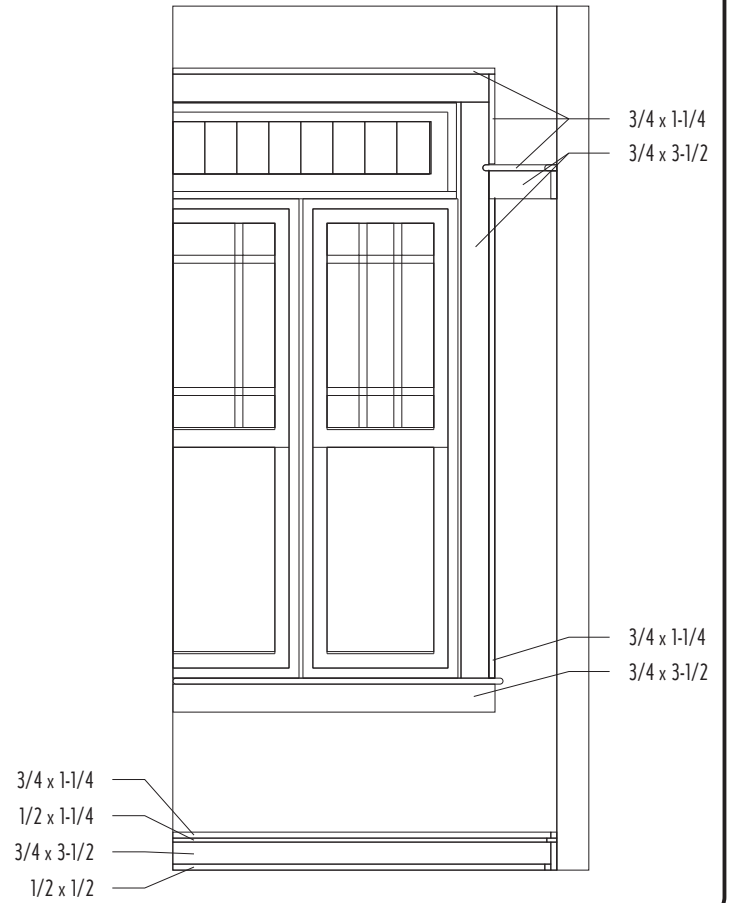
Interior Trim Detail (Typical)
